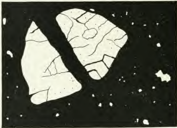
Fig. 22—Character of ore at Creighton mine, Sudbury area, Ontario, ninth level, near hanging wall. White represents greenstone boulders; black represents sulphides. Width of face 4\frac{1}{2} feet.
